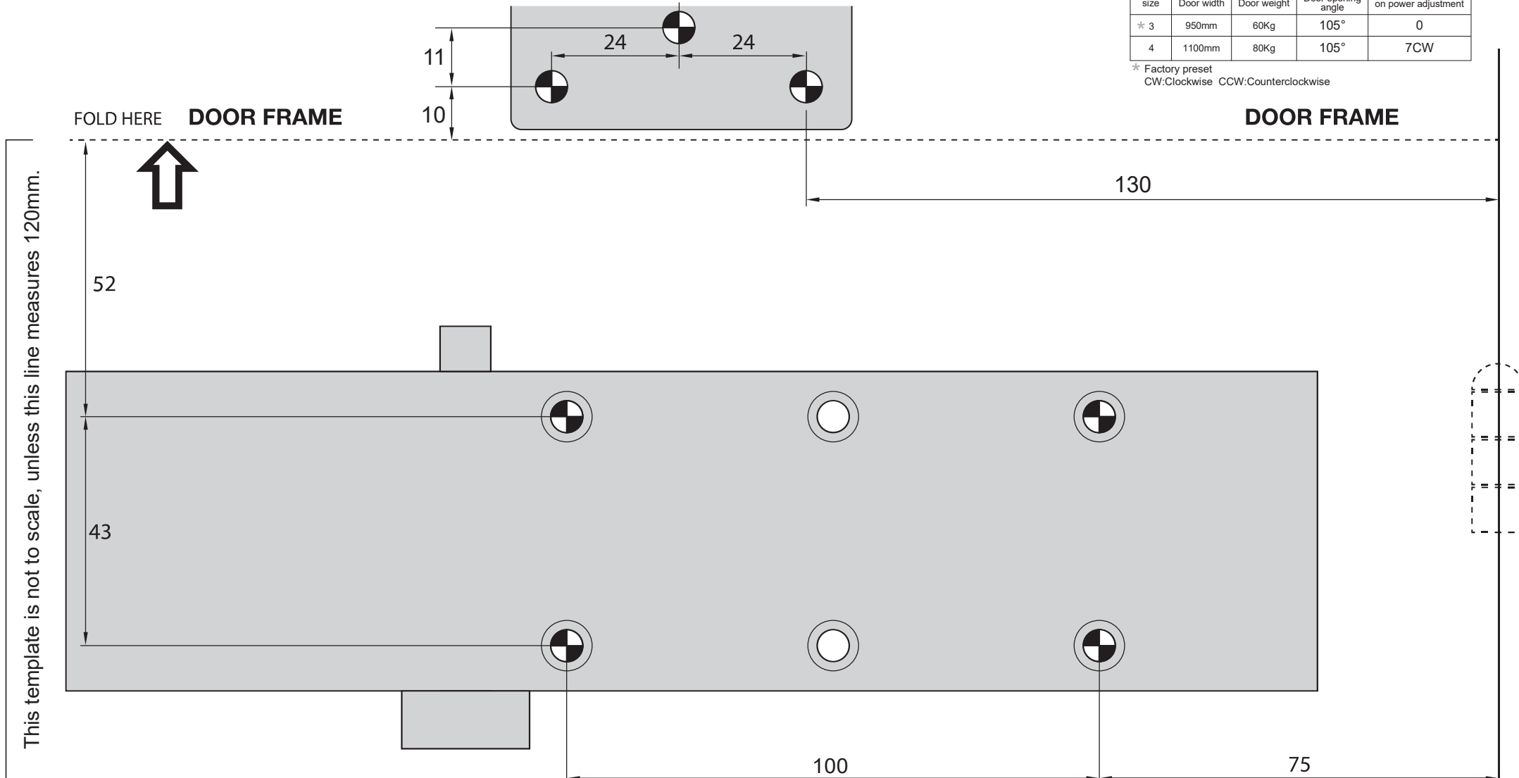
Figure 6 Fixing
