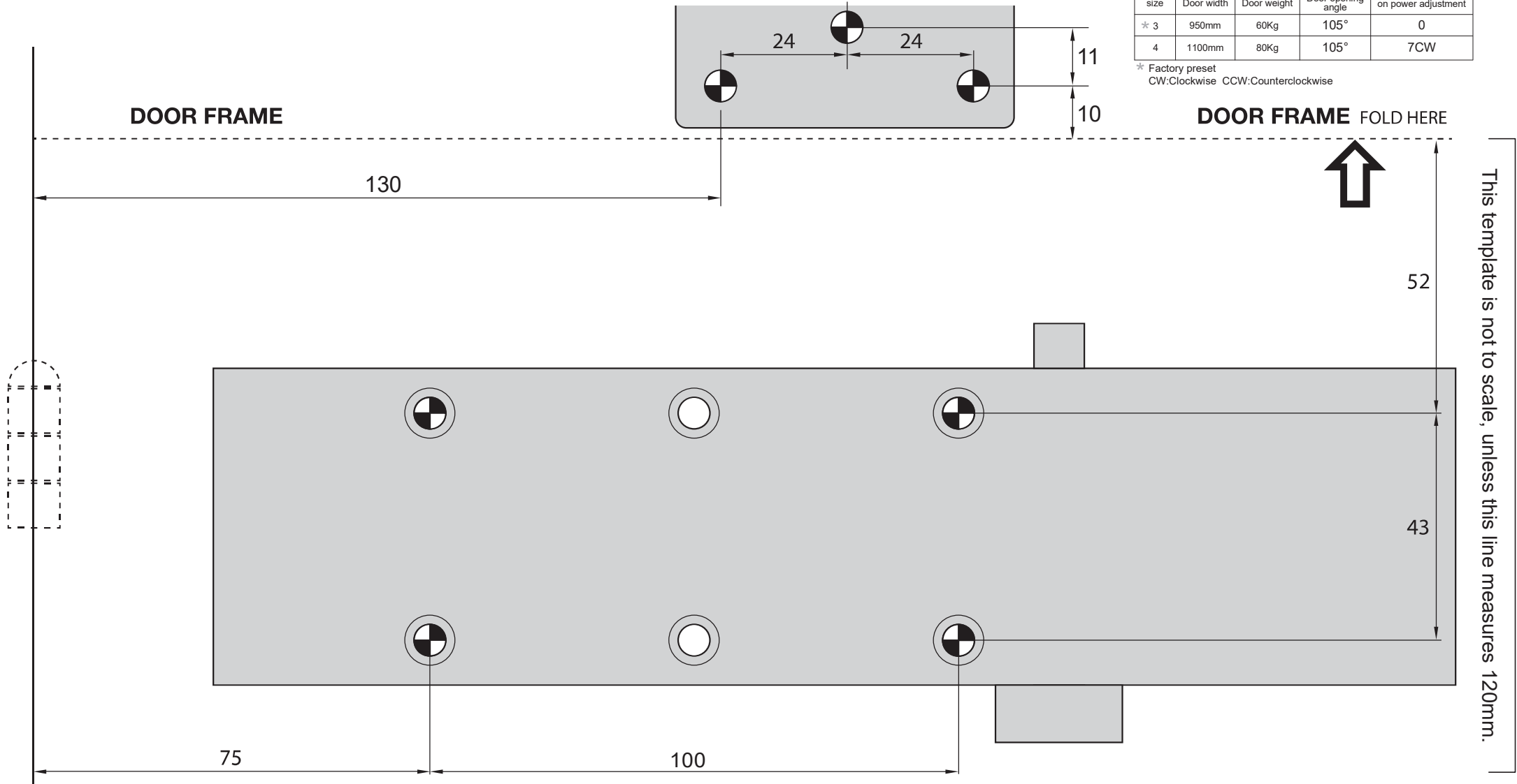
Figure 6 Fixing
